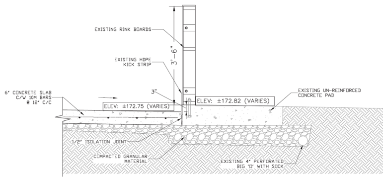
Option 1 - Draft Concrete Slab Layout
