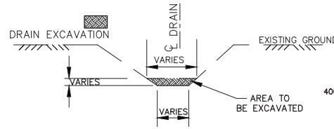
TYPICAL DRAIN CROSS SECTION STATION 0+014 TO 0+070 NTS
