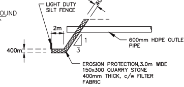
OUTLET DETAIL NTS
