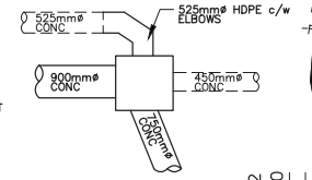
JUNCTION BOX #1 DETAIL NTS
